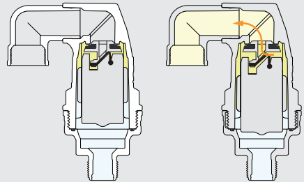
Pipe is full of water
